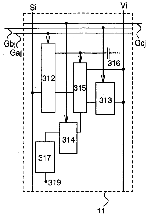
FIG. 11D
