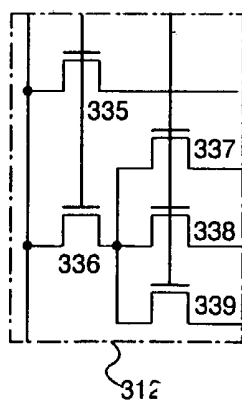
FIG. 12D
