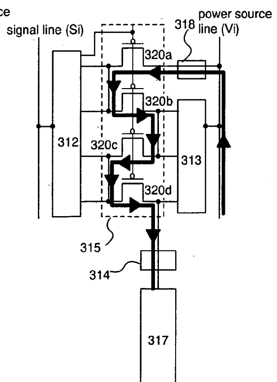
FIG. 11D
